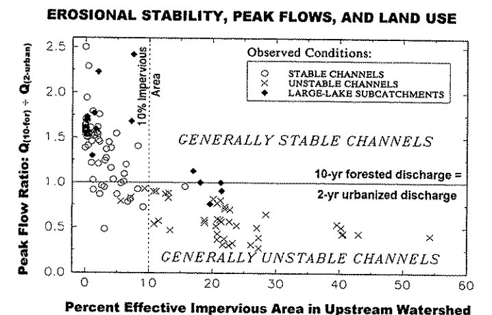
Figure 7. Observed stable ("O") and unstable ("X") channels, plotted by percent effective impervious area (EIA) in the upstream watershed (horizontal scale) and ratio of modeled ten-year forested and two-year urbanized (i.e., current) discharges (vertical scale). "Stable channels" consistently meet the apparent thresholds of either ( EIA \leq 10 percent) or ( Q_{2-urban} \leq Q_{10-for} ), except for the few catchments containing large lakes (from Booth and Jackson, 1997).
