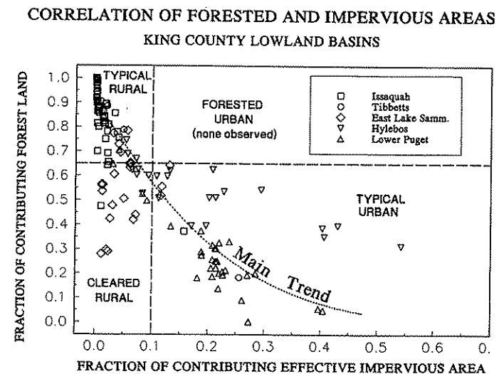
Figure 10. Land cover data from individual subcatchments within five King County watersheds, compiled from Basin Plan land-cover data (King County, 1990c, 1990e, 1991). At 65-percent forest retention, EIA \leq 10 percent in all cases, yet with EIA < 10 percent, substantial clearing is still commonly observed.
