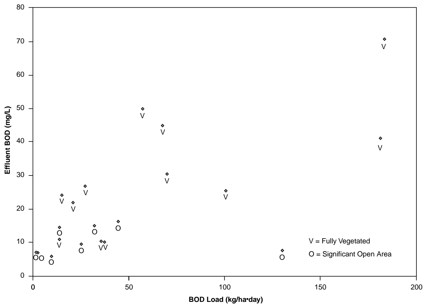
Figure 4-1. BOD effluent vs. areal loading (DMDB)
