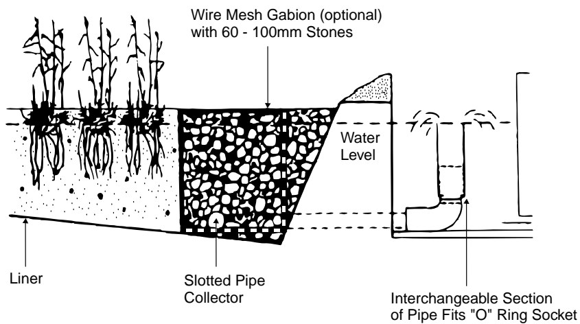
b) Interchangeable Section
