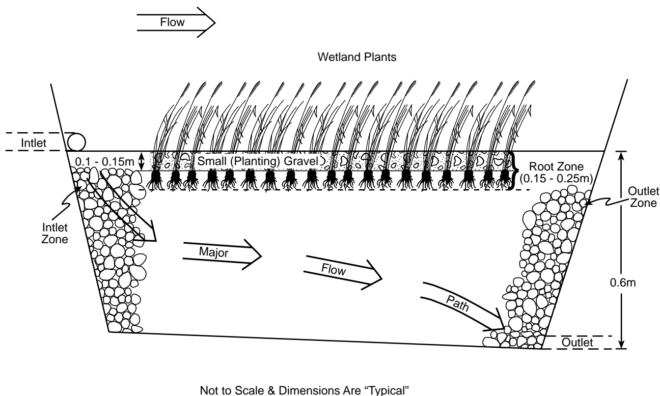
Figure 5-2. Preferential Flow in a VSB
