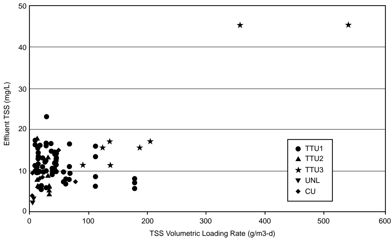
Figure 5-5. Effluent TSS vs volumetric loading rate
