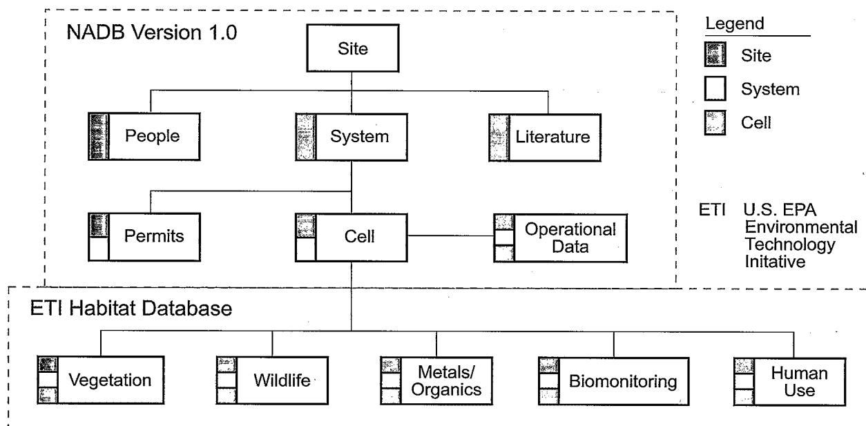
File structure of the North American Treatment Wetland System Database Version 2.0.
