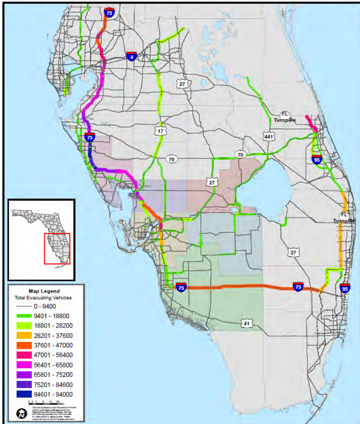
Figure G-2 Evacuation Trip Volumes for 2015 Operational Scenario 2 Evacuation Level B
