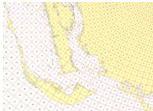
Figure II-2: SLOSH Grid With Surge Values
