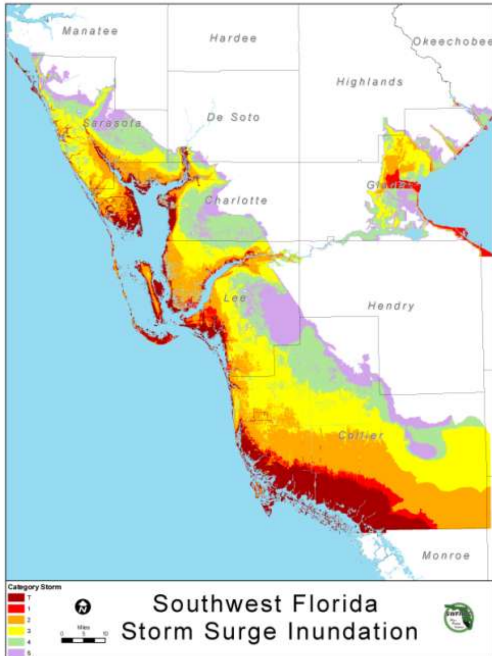
FIGURE II-3 SOUTHWEST REGION STORM TIDE MAP
