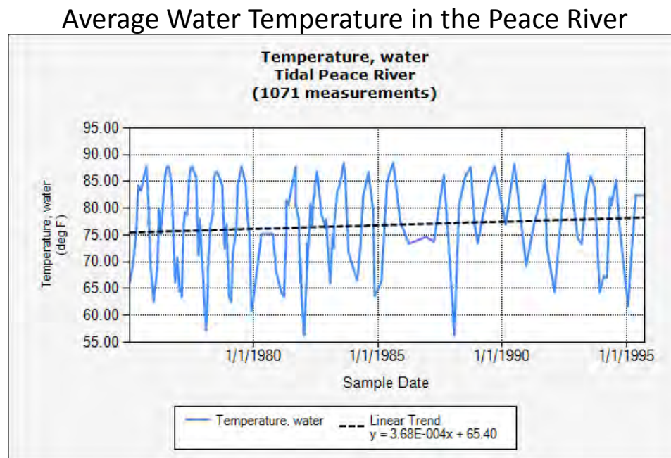
Figure 129: Average Water Temperature of the Peace River
