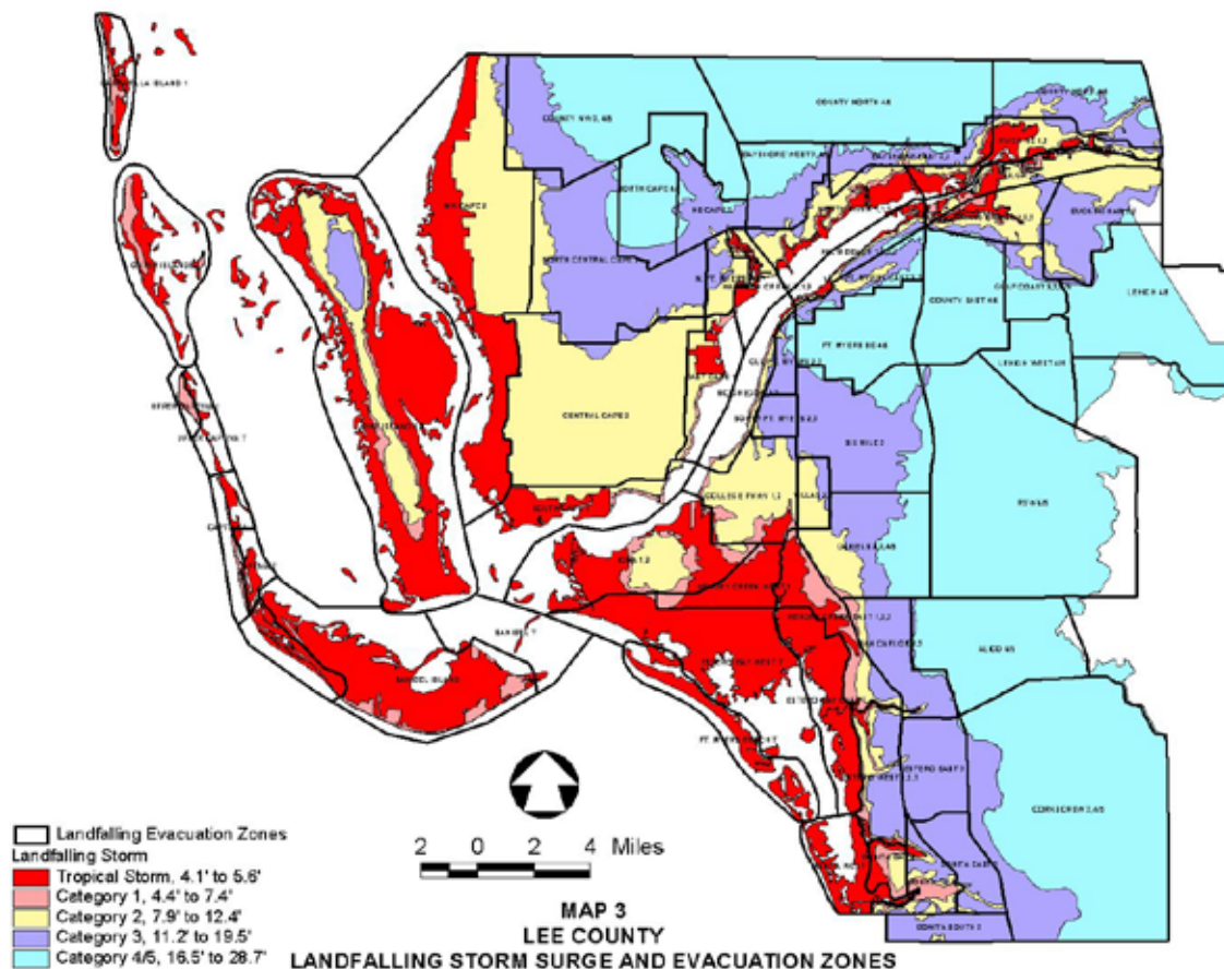
Figure 6: Current Storm Surge Boundaries for Lee County
