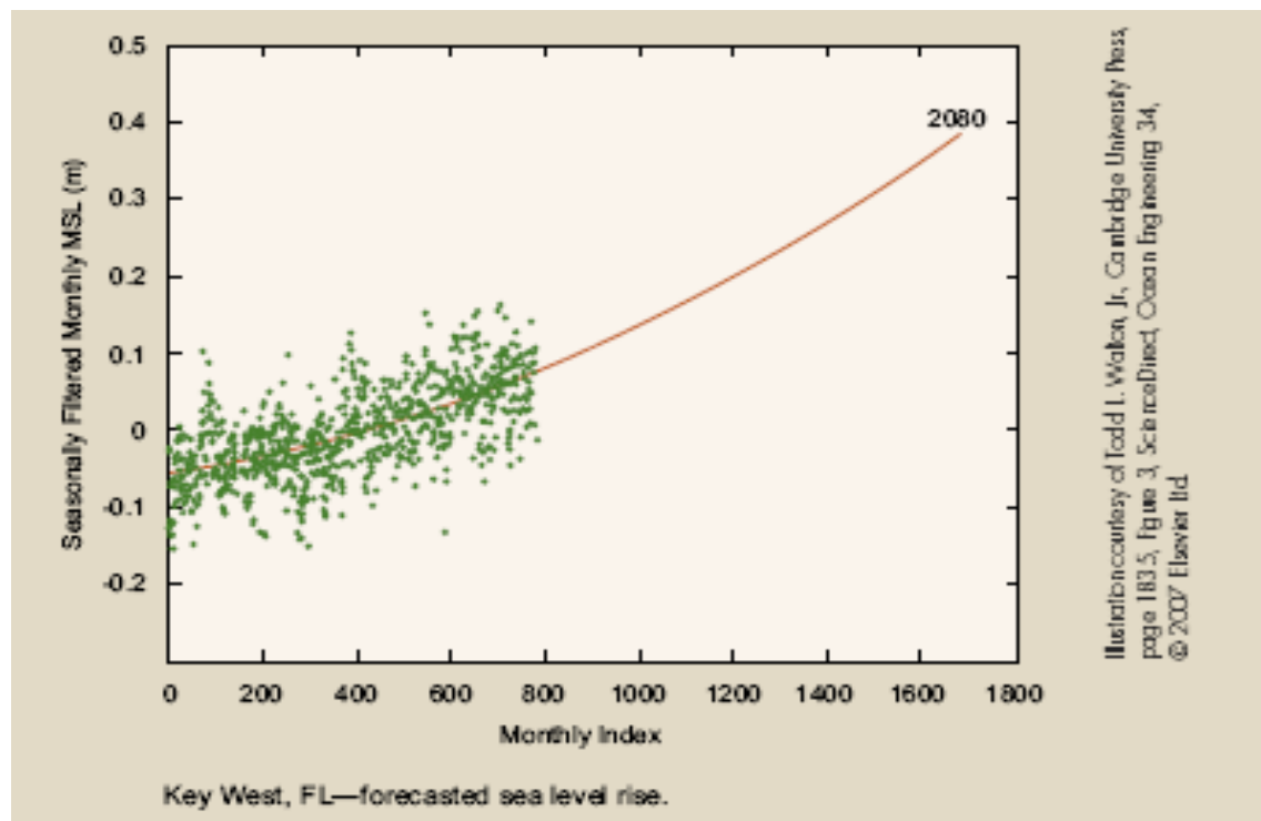
Figure 19: Forecasted Sea Level Rise at Key West, Florida
