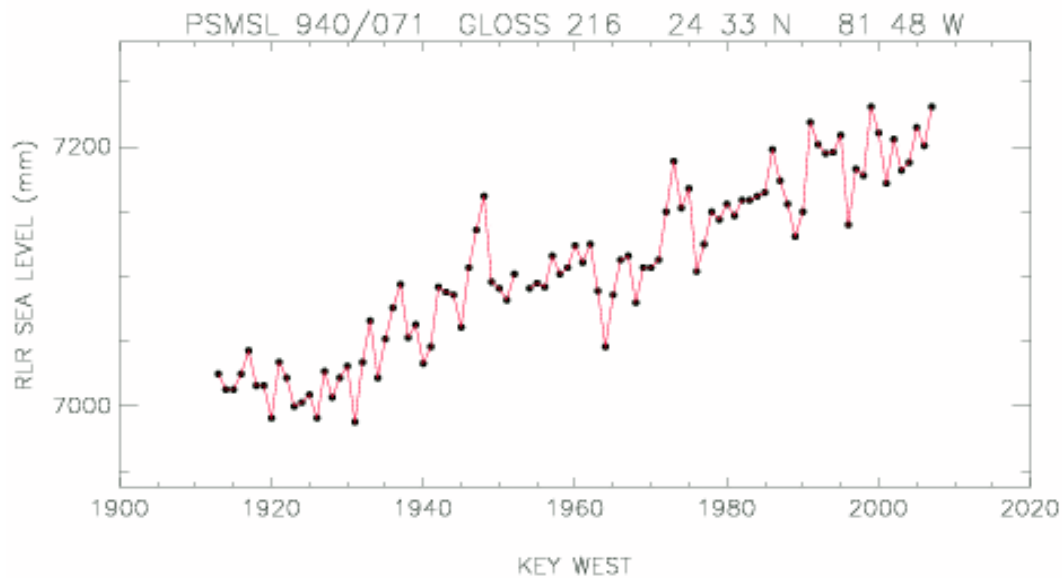
Figure 17: Mean Annual Sea Level at Key West, Florida 1910-2009
